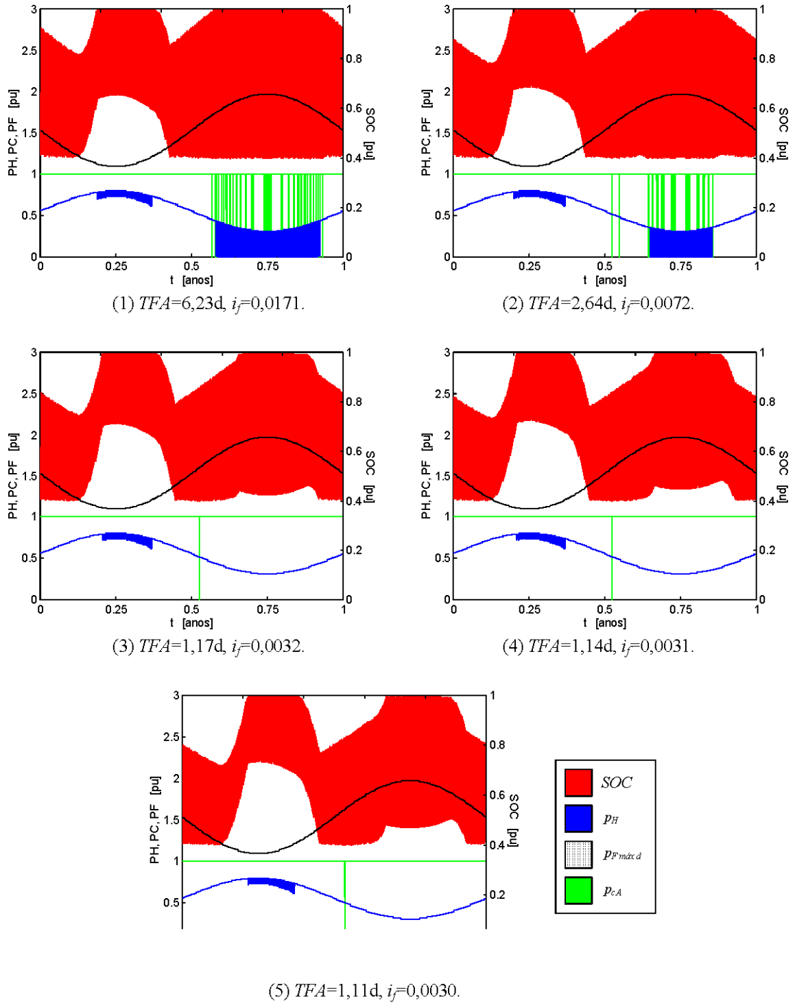
FIGURE 2. Effects of different dimensions of bank of batteries on the performance of a system with p_{dd}=1,00 , \kappa_t=1,00 , \kappa_e=1,00 [ p_{sh}=1,00 ], \kappa_a=1,00 [ p_{Mm}=1,00 , df=1,1496 , dh=df ], \kappa=1,00 , with p_{he\ máx}=p_{c\ máx} and a_f=24,61 , without water reservoir and with constant load demand profile. Banks of batteries with capacity for (1) 0,500 day, (2) 0,550 day, (3) 0,600 day, (4) 0,625 day and (5) 0,650 day, with discharge until 40% and charge until 100% of maximum capacity. Conventions: SOC: state of charge of the batteries, p_H : power made available by the hydro generator set, p_F^{máx d} : maximum daily power made available by the PV generator set, p_{cA} : power delivered to the loads.
